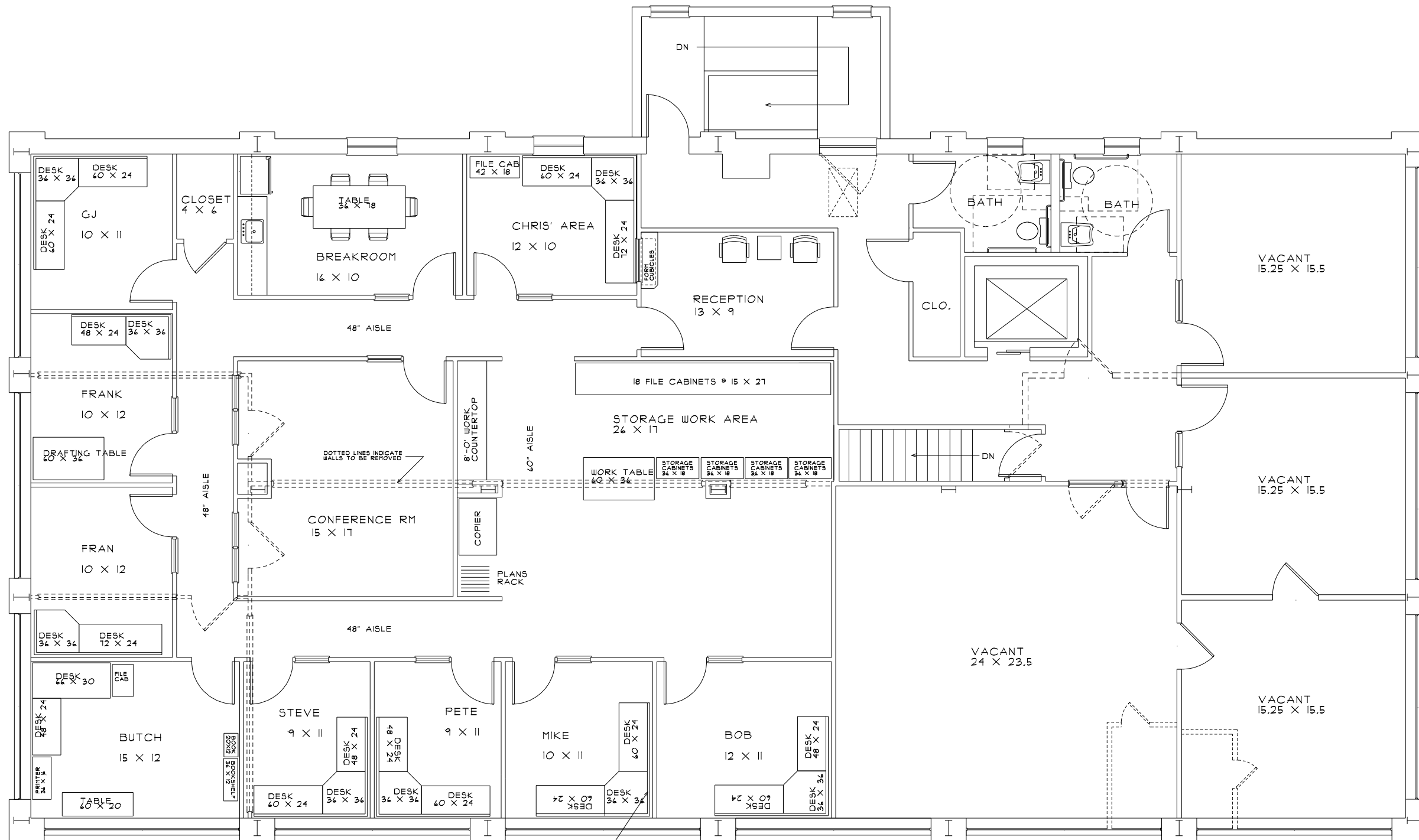
THIRD FLOOR PLAN SCALE: 1/8" = 1'-0"
